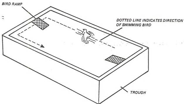
WILDLIFE LADDER, BIRD RAMP AT A 45° ANGLE TO TROUGH DOES NOT INTERCEPT LINE OF TRAVEL
